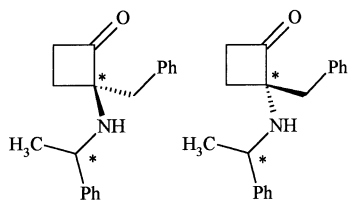
Figure 2. The rearranged \alpha -amino ketones
