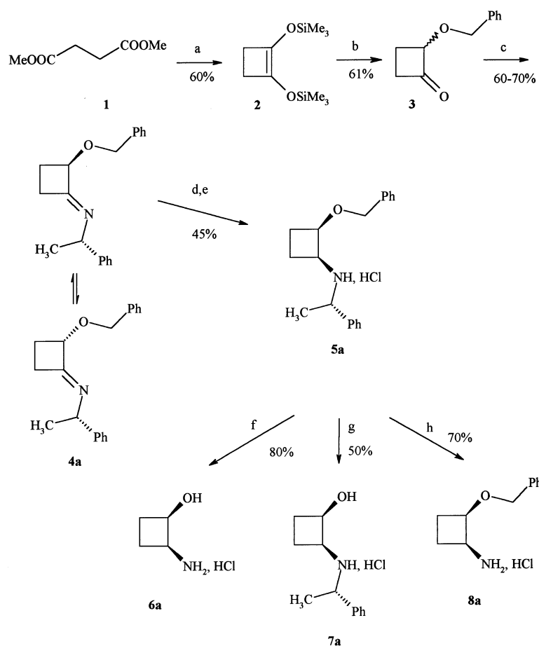
Scheme 2. Synthesis of the optically active 6a , 7a and 8a (the same procedure applies for the synthesis of 6b , 7b and 8b )
