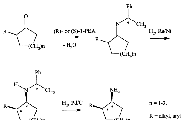
Scheme 1. Asymmetric reductive amination sequence
