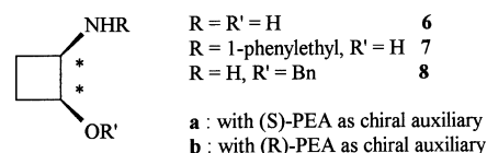
Figure 1. The (+)- and (–)- cis -2-aminocyclobutanols and corresponding benzyloxycyclobutanamines
